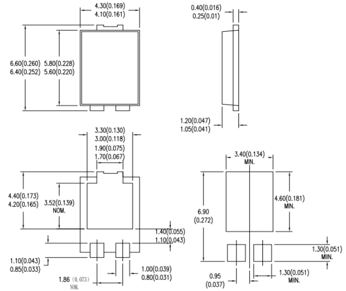
TO-277B
